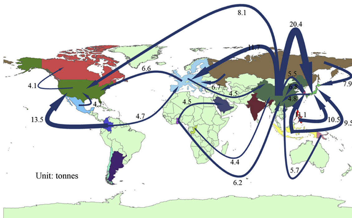
Fig. 3. Embodied mercury fluxes ( \geq 4 tonnes) between trading centers.
