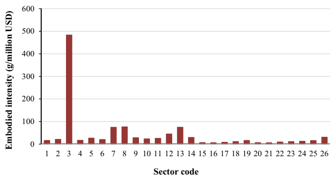
Fig. 2. Sectoral embodied nonferrous metal related mercury emission intensities.
